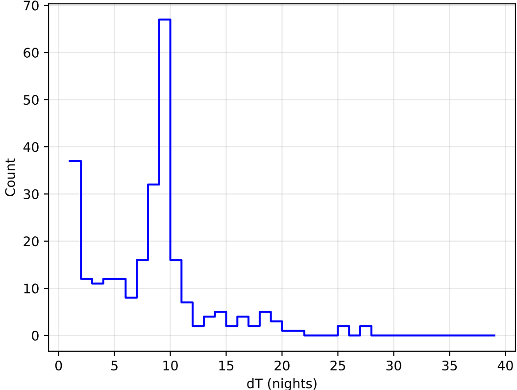
too_elab_heavy_r64_d3_ugrizy_v3.4_10yrs all bands: DD:ELAISS1 Delta Nights Histogram
