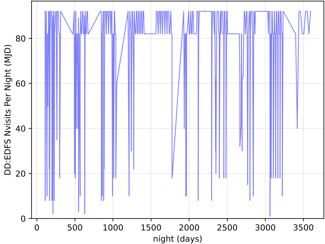
too_elab_heavy_r64_d3_ugrzyz_v3.4_10yrs all bands: DD:EDFS Nvisits Per Night
