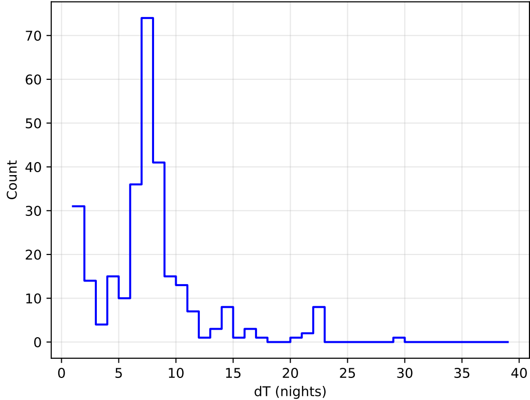
too_elab_heavy_r64_d3_ugrizy_v3.4_10yrs all bands: DD:EDFS Delta Nights Histogram
