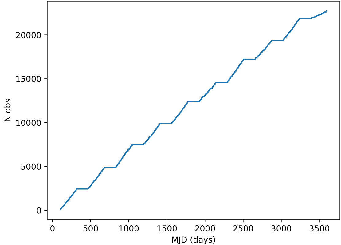
too_elab_heavy_r64_d3_ugrizy_v3.4_10yrs all bands: DD:EDFS Cumulative NVisits
