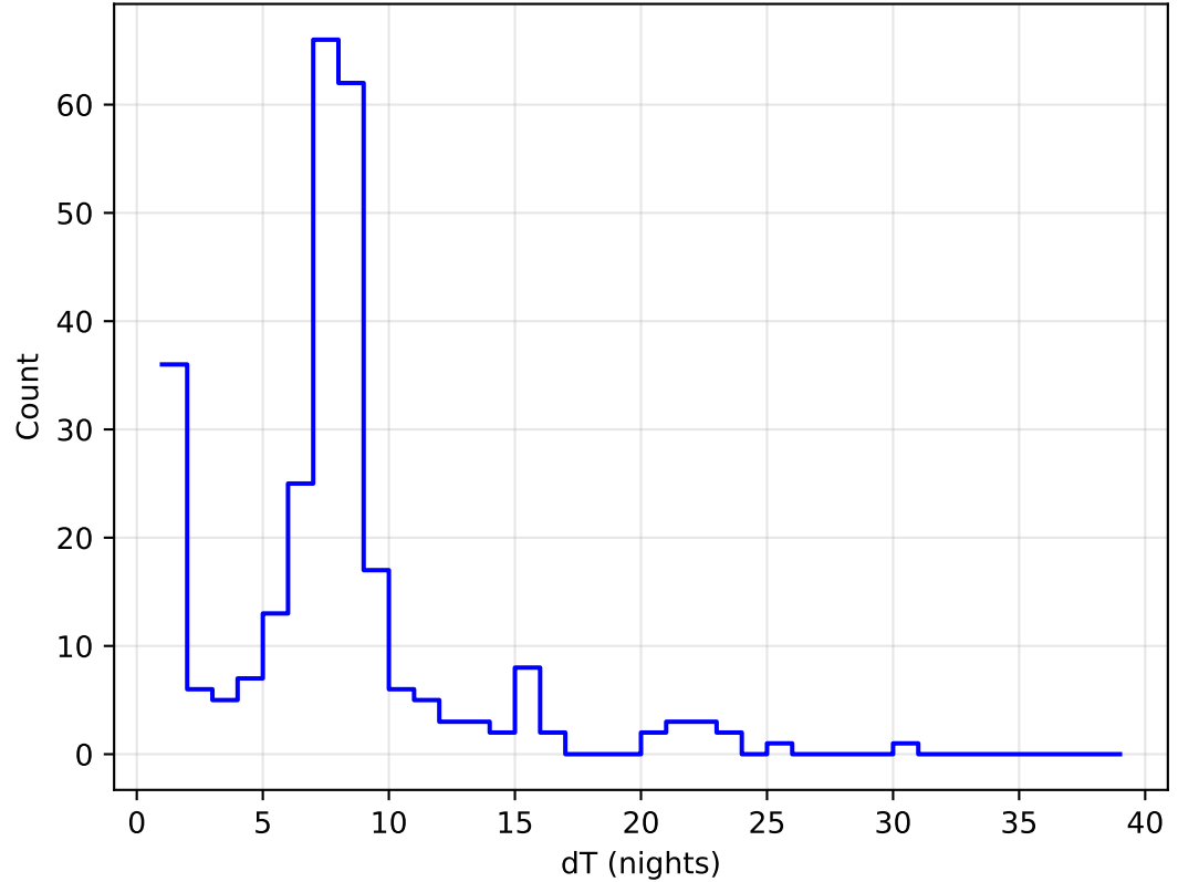
too_elab_heavy_r64_d3_ugrizy_v3.4_10yrs all bands: DD:ECDFS Delta Nights Histogram
