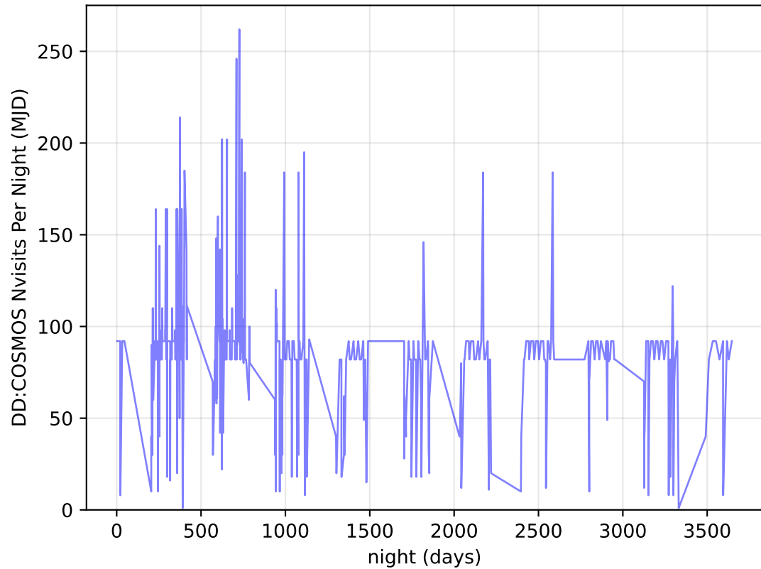
too_elab_heavy_r64_d3_ugrizy_v3.4_10yrs all bands: DD: COSMOS Nvisits Per Night
