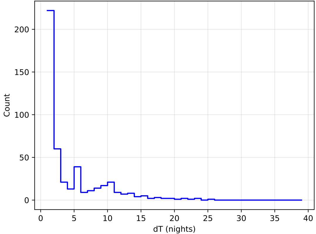
too_elab_heavy_r64_d3_ugrizy_v3.4_10yrs all bands: DD: COSMOS Delta Nights Histogram
