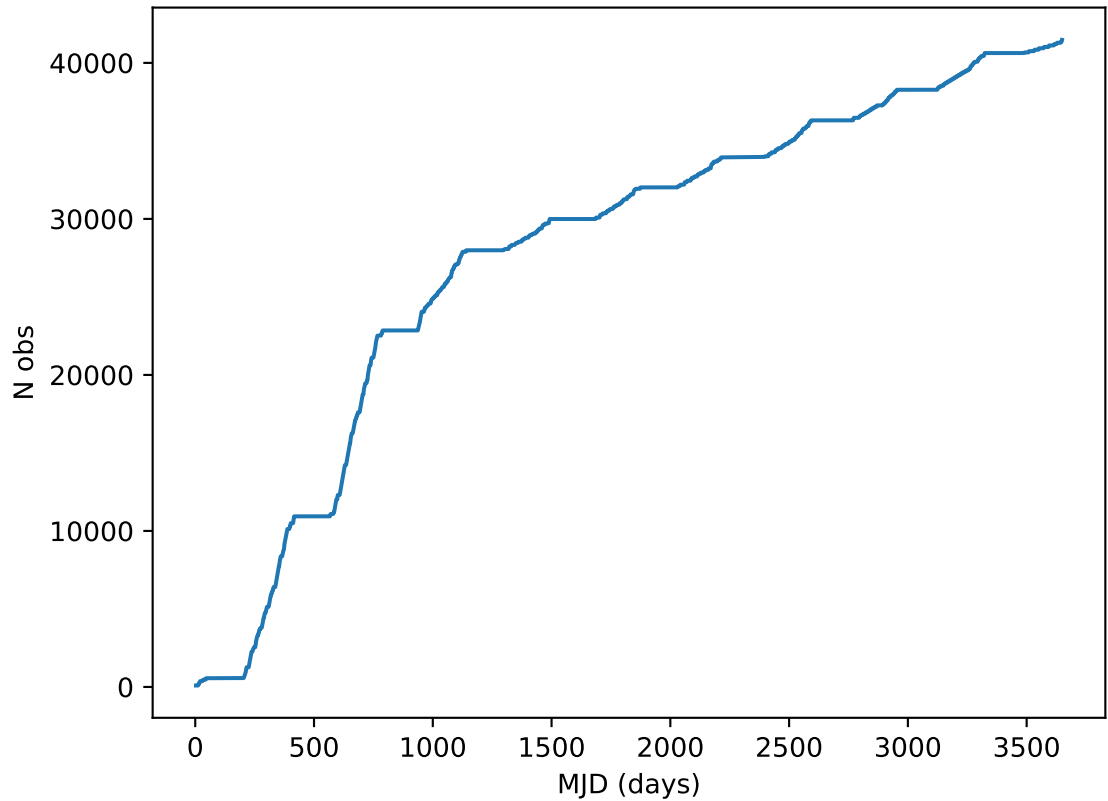
too_elab_heavy_r64_d3_ugrizy_v3.4_10yrs all bands: DD: COSMOS Cumulative NVisits
