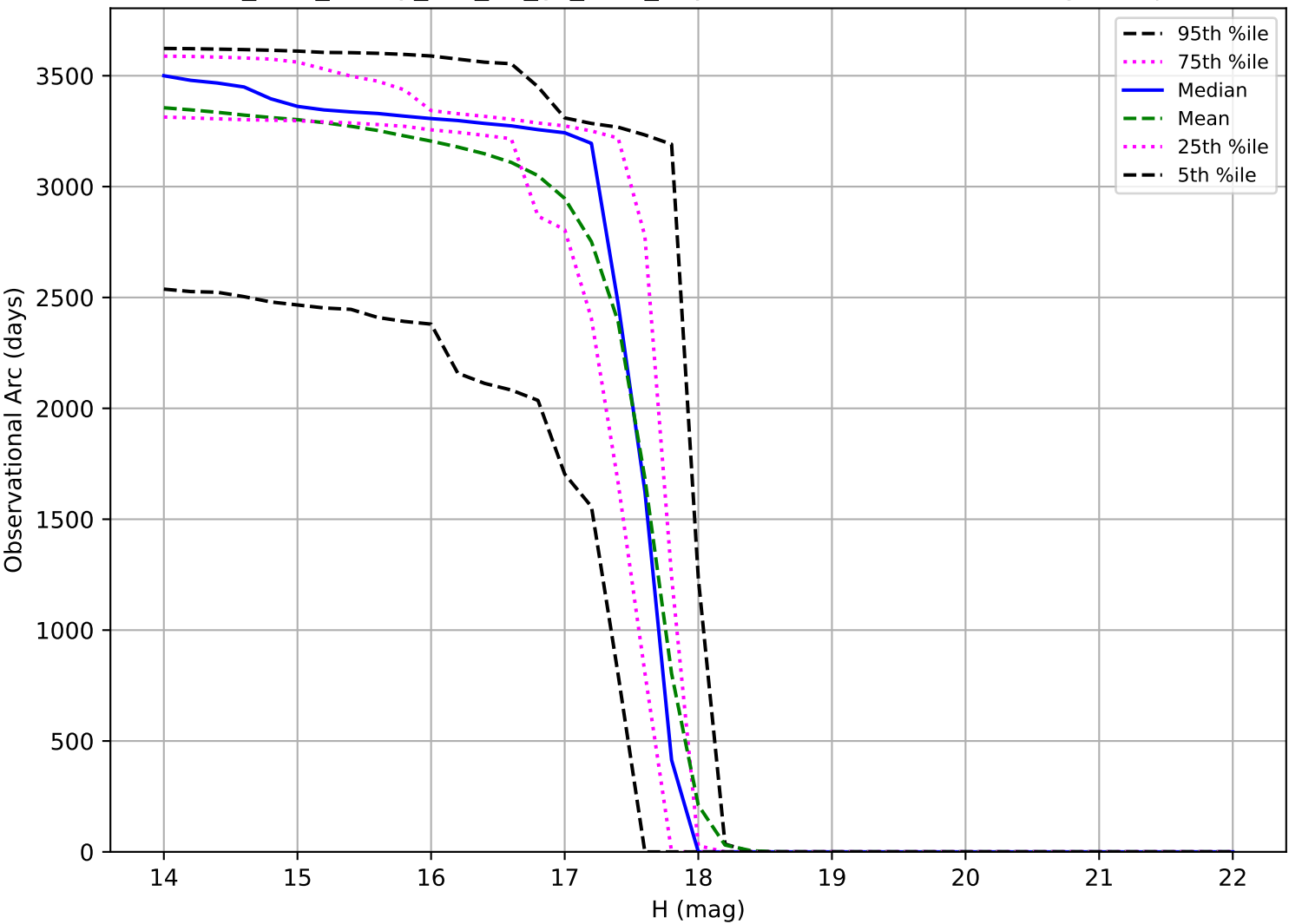
too_elab_heavy_r64_d3_gz_v3.4_10yrs: Observational Arc Length Trojan
