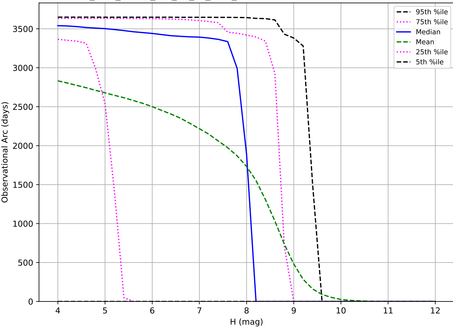
too_elab_heavy_r64_d3_gz_v3.4_10yrs: Observational Arc Length TNO
