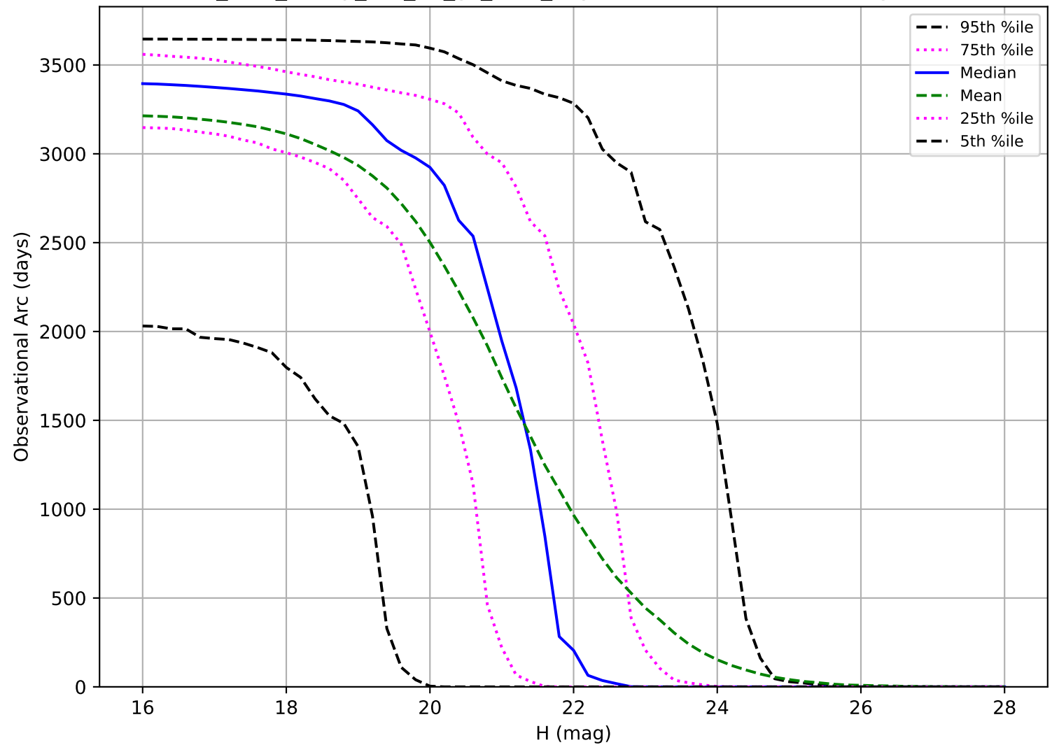
too_elab_heavy_r64_d3_gz_v3.4_10yrs: Observational Arc Length PHA
