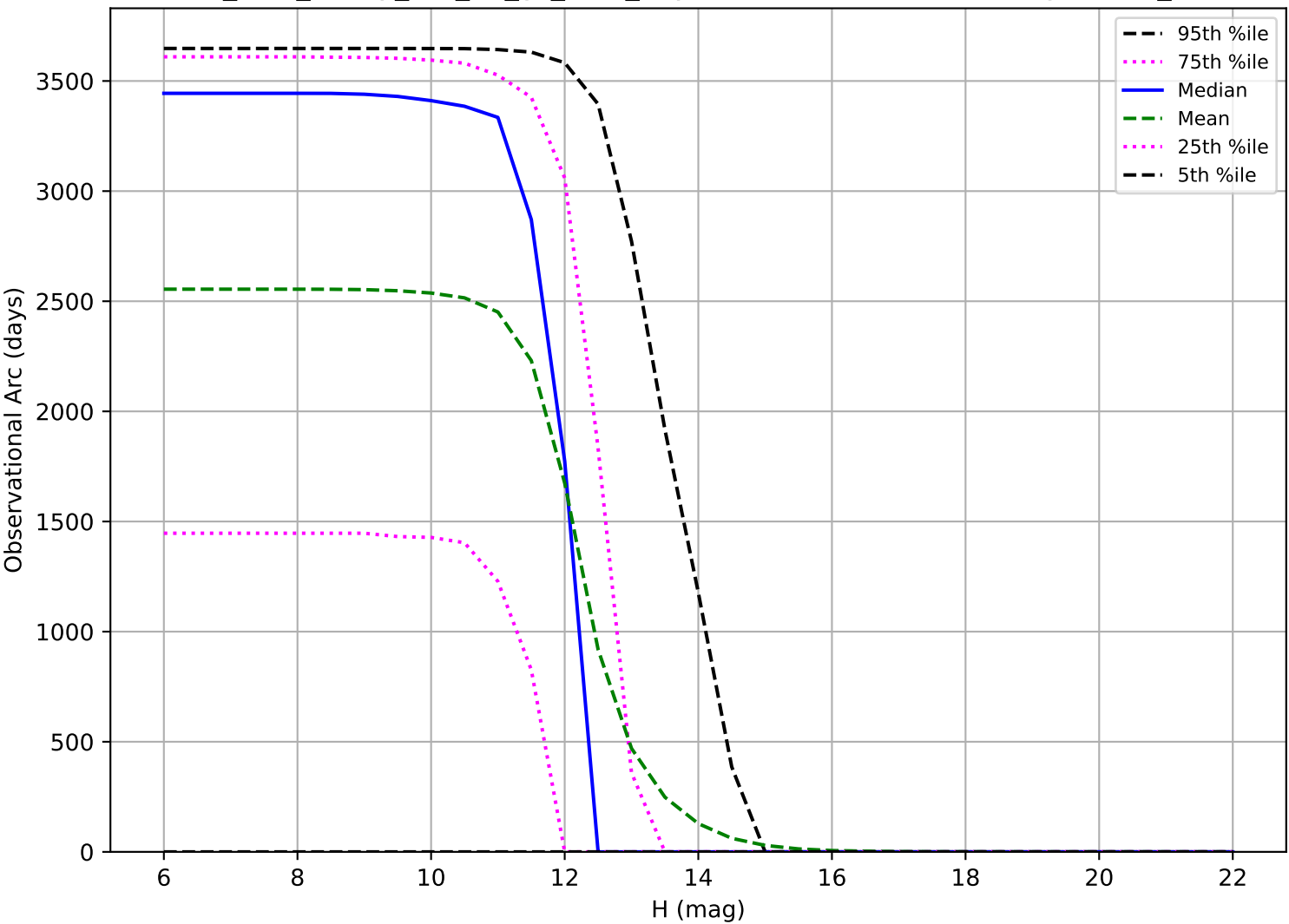
too_elab_heavy_r64_d3_gz_v3.4_10yrs: Observational Arc Length OCC_r20
