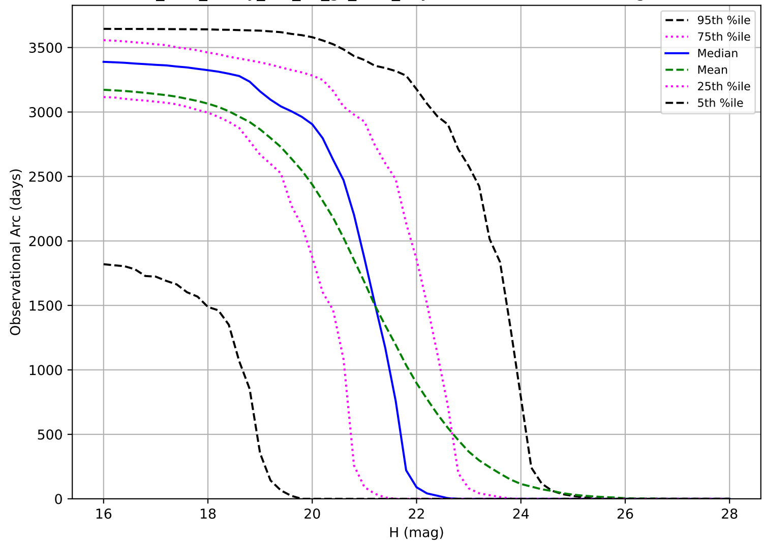
too_elab_heavy_r64_d3_gz_v3.4_10yrs: Observational Arc Length NEO
