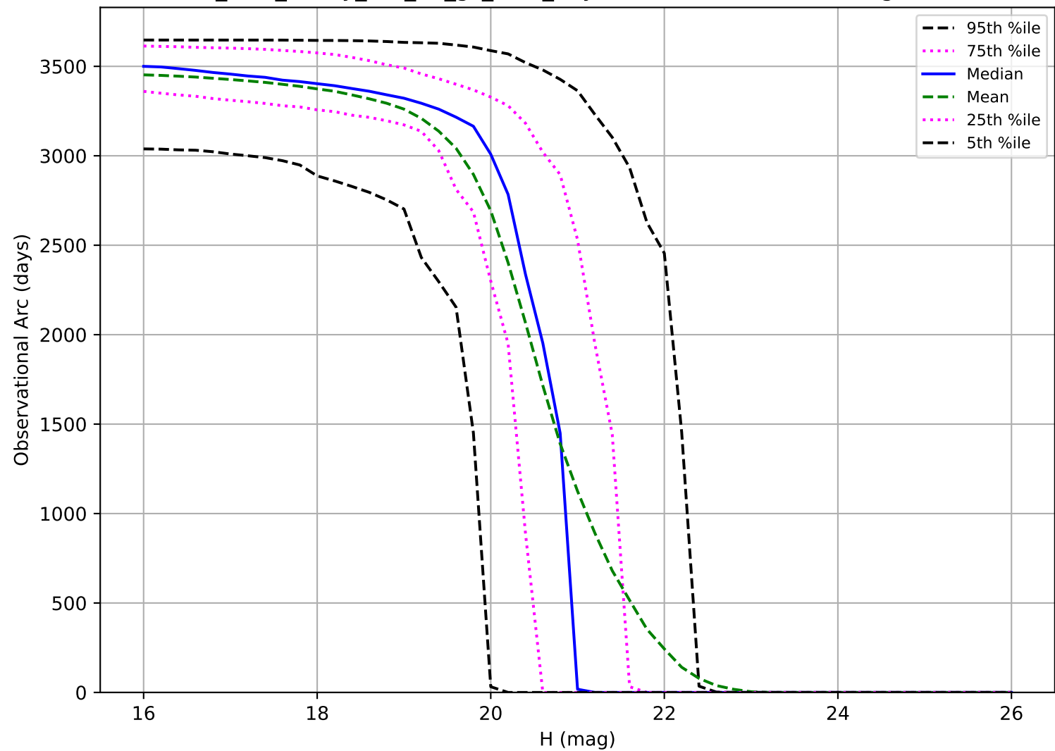
too_elab_heavy_r64_d3_gz_v3.4_10yrs: Observational Arc Length MBA
