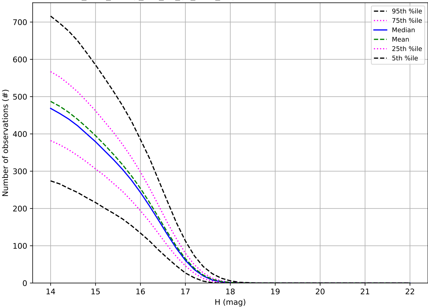
too_elab_heavy_r64_d3_gz_v3.4_10yrs: Number of observations Trojan
