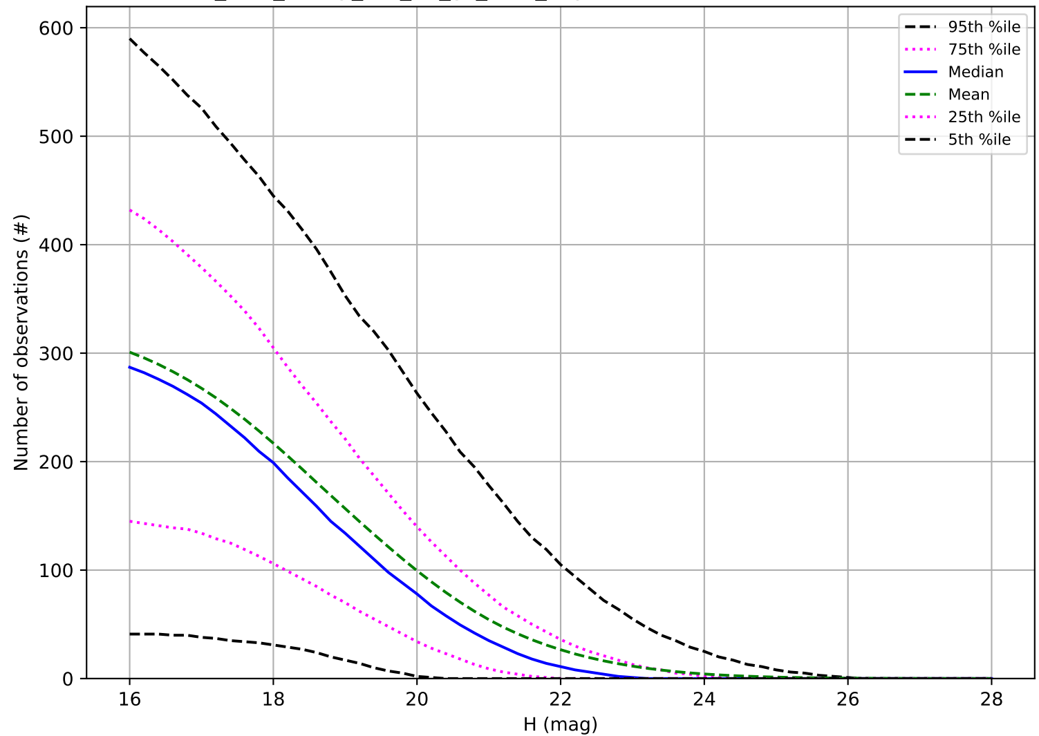
too_elab_heavy_r64_d3_gz_v3.4_10yrs: Number of observations PHA
