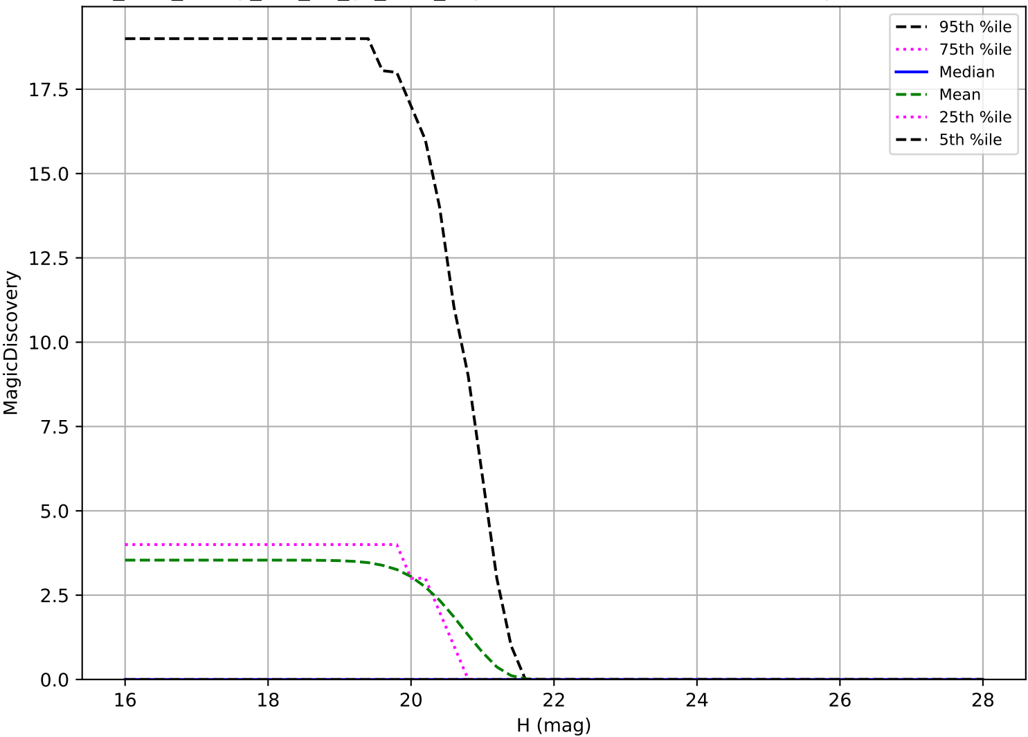
too_elab_heavy_r64_d3_gz_v3.4_10yrs: Vatira 6 detections in 60 nights detection loss
