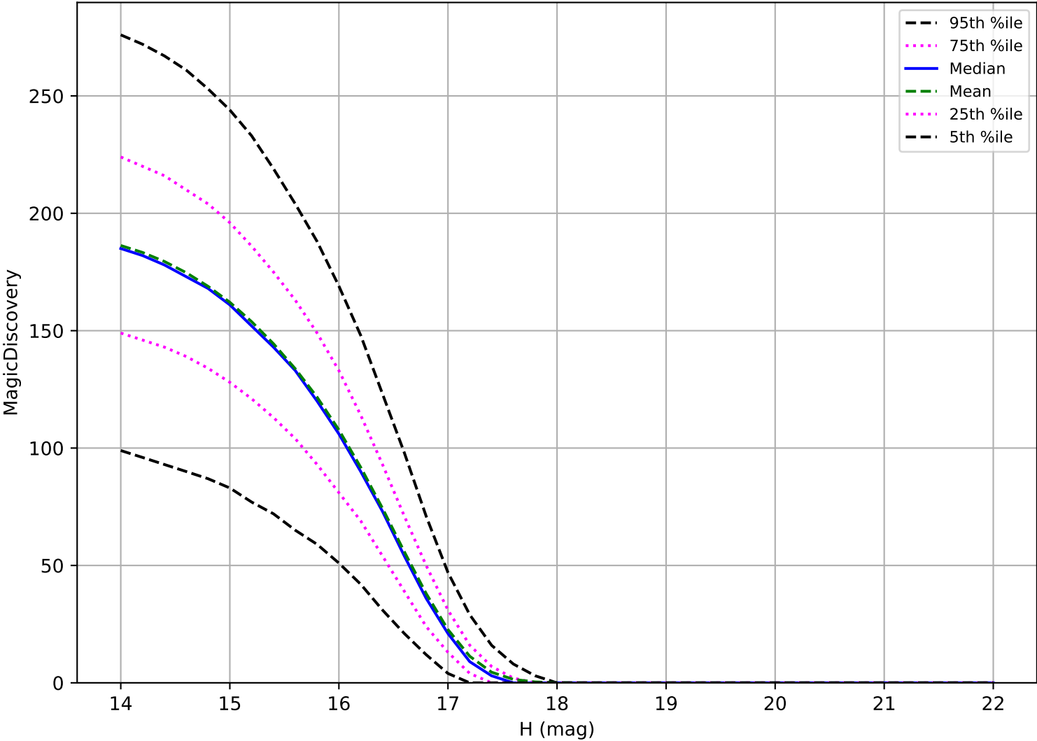
too_elab_heavy_r64_d3_gz_v3.4_10yrs: Trojan 6 detections in 60 nights detection loss
