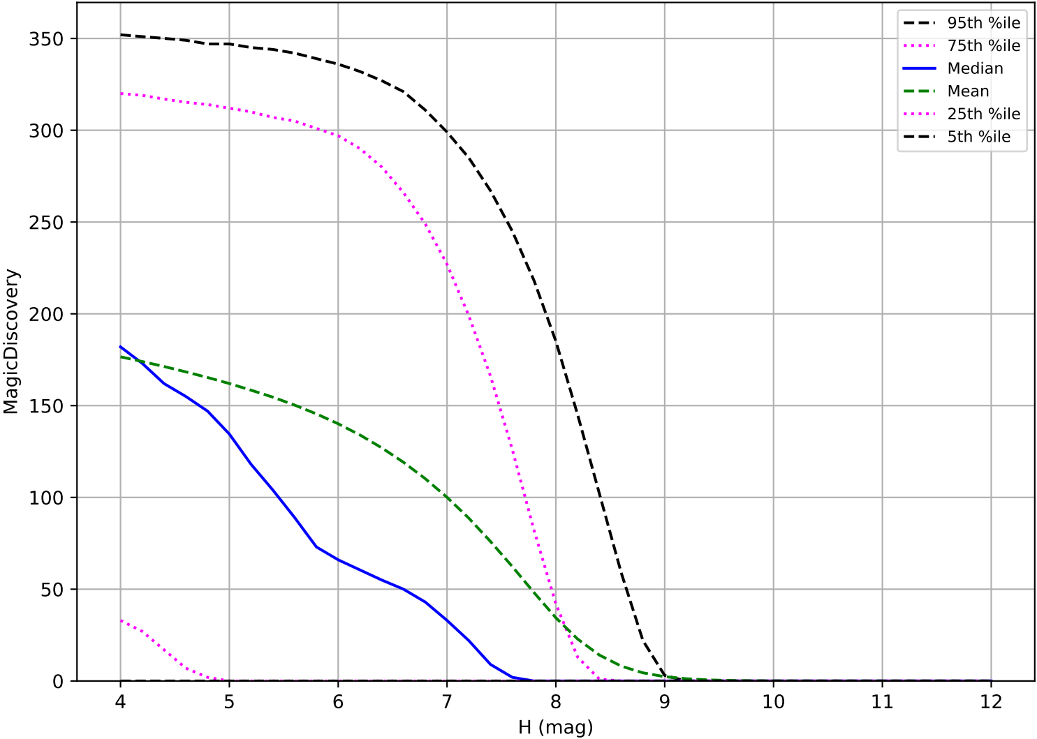
too_elab_heavy_r64_d3_gz_v3.4_10yrs: TNO 6 detections in 60 nights detection loss
