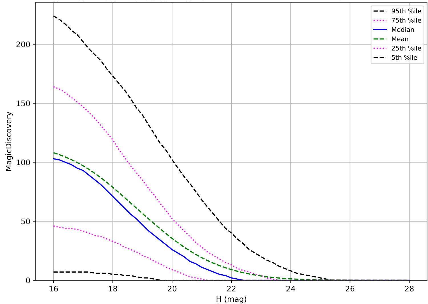
too_elab_heavy_r64_d3_gz_v3.4_10yrs: PHA 6 detections in 60 nights detection loss
