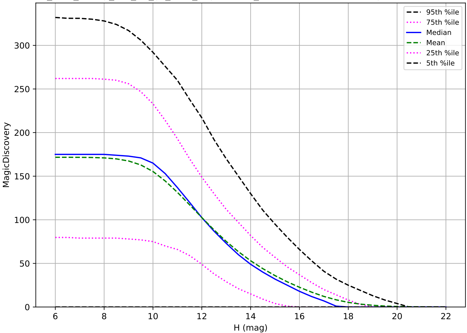
too_elab_heavy_r64_d3_gz_v3.4_10yrs: OCC_r5 6 detections in 60 nights detection loss
