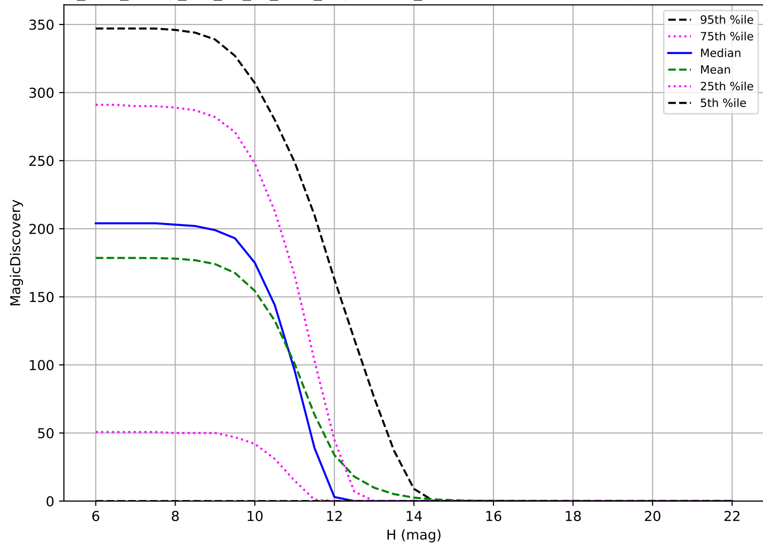
too_elab_heavy_r64_d3_gz_v3.4_10yrs: OCC_r20 6 detections in 60 nights detection loss
