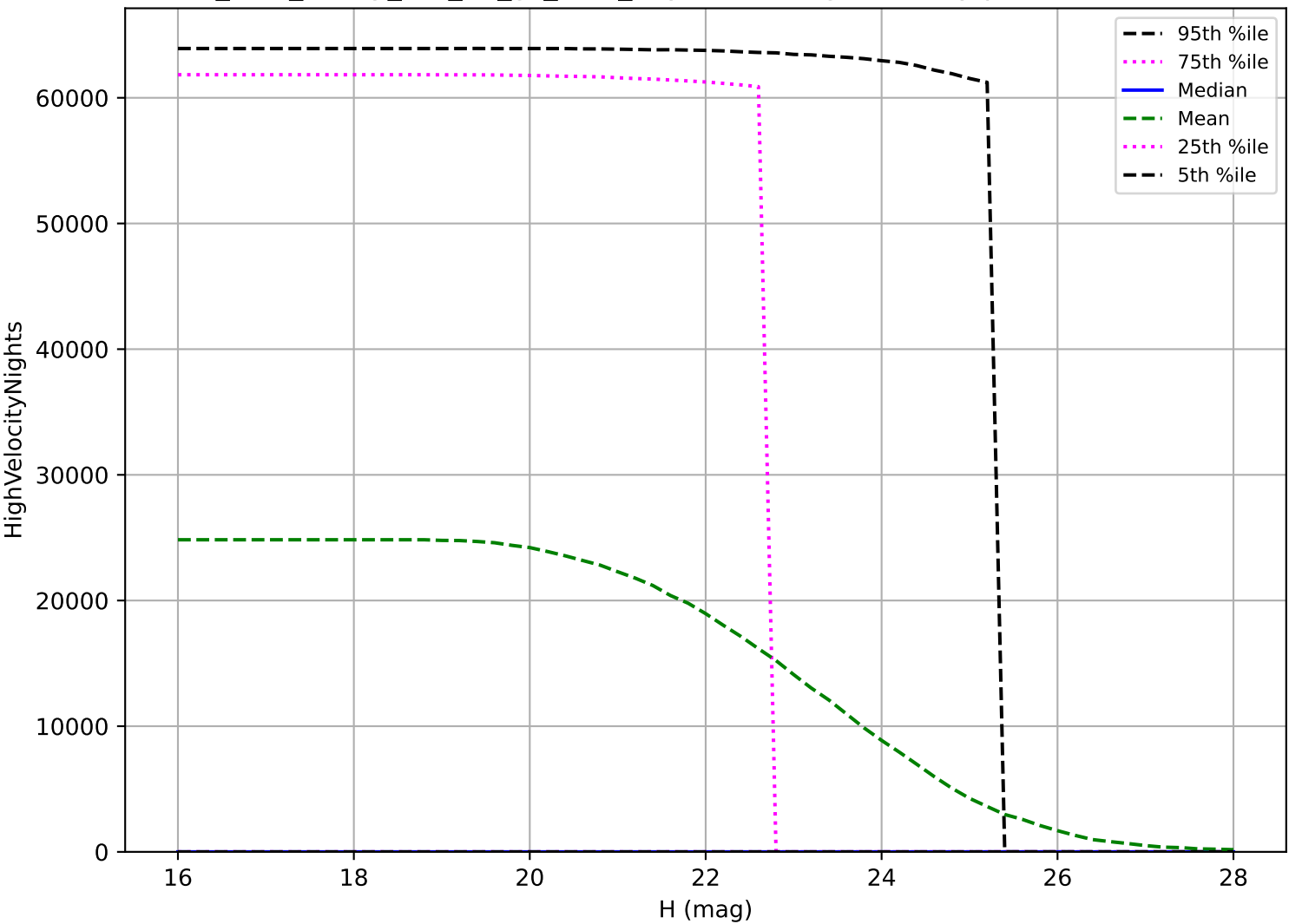
too_elab_heavy_r64_d3_gz_v3.4_10yrs: PHA High velocity pair detection loss
