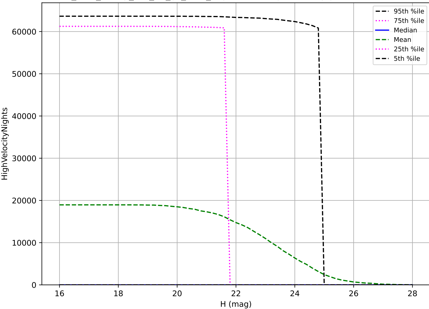
too_elab_heavy_r64_d3_gz_v3.4_10yrs: NEO High velocity pair detection loss
