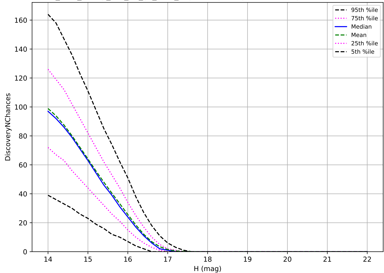
too_elab_heavy_r64_d3_gz_v3.4_10yrs: Trojan 3 pairs in 15 nights detection loss
