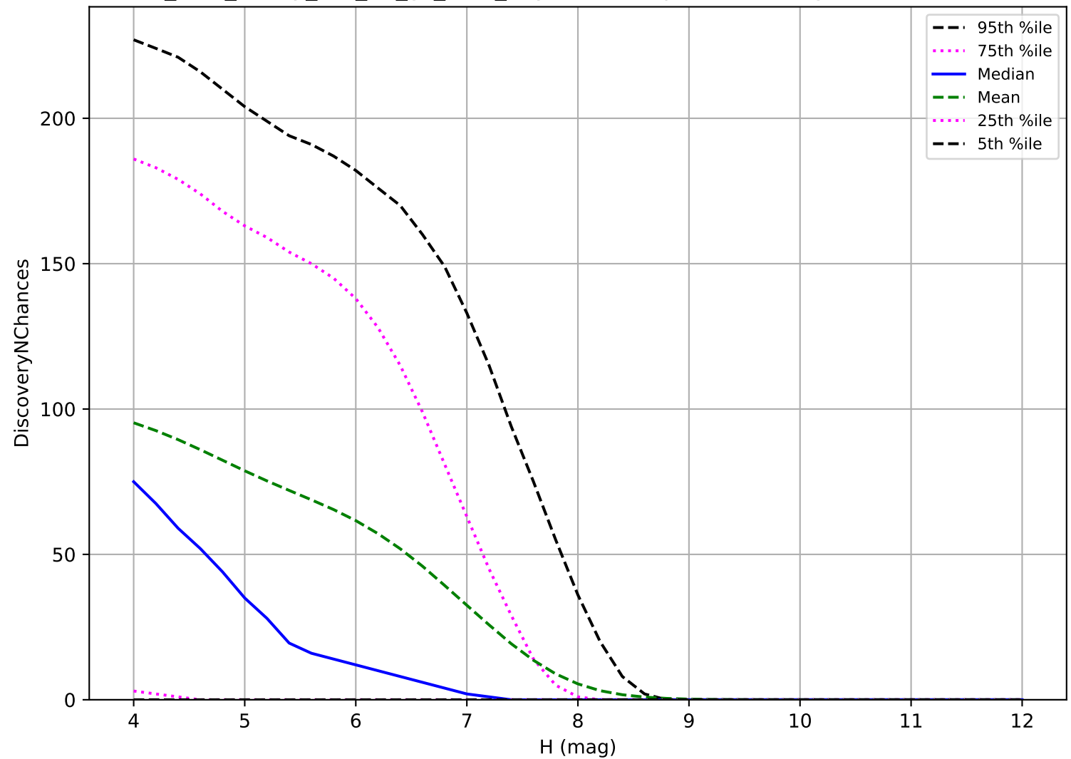
too_elab_heavy_r64_d3_gz_v3.4_10yrs: TNO 3 pairs in 15 nights detection loss
