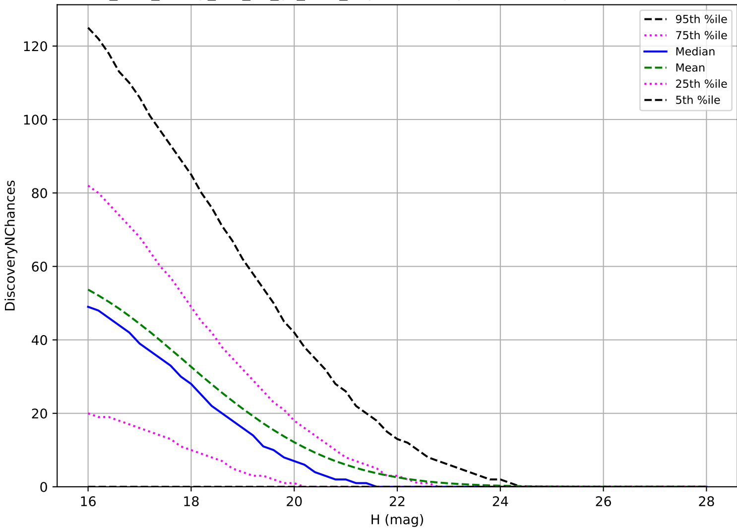
too_elab_heavy_r64_d3_gz_v3.4_10yrs: NEO 3 pairs in 15 nights detection loss
