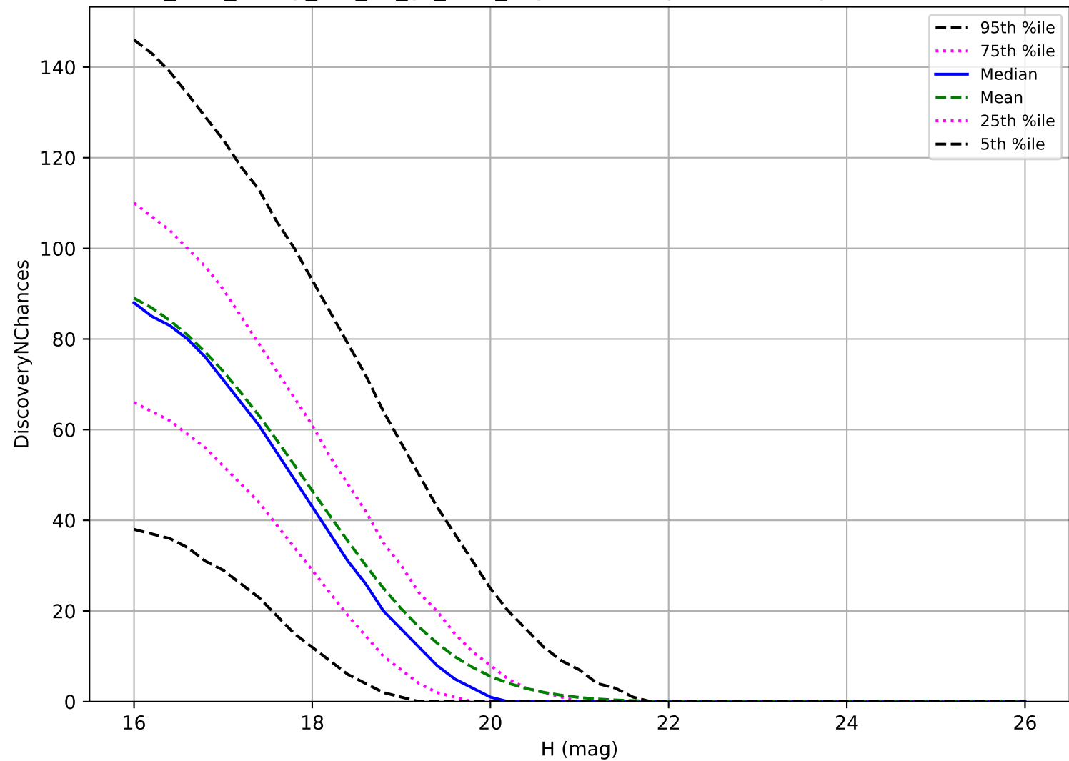
too_elab_heavy_r64_d3_gz_v3.4_10yrs: MBA 3 pairs in 15 nights detection loss
