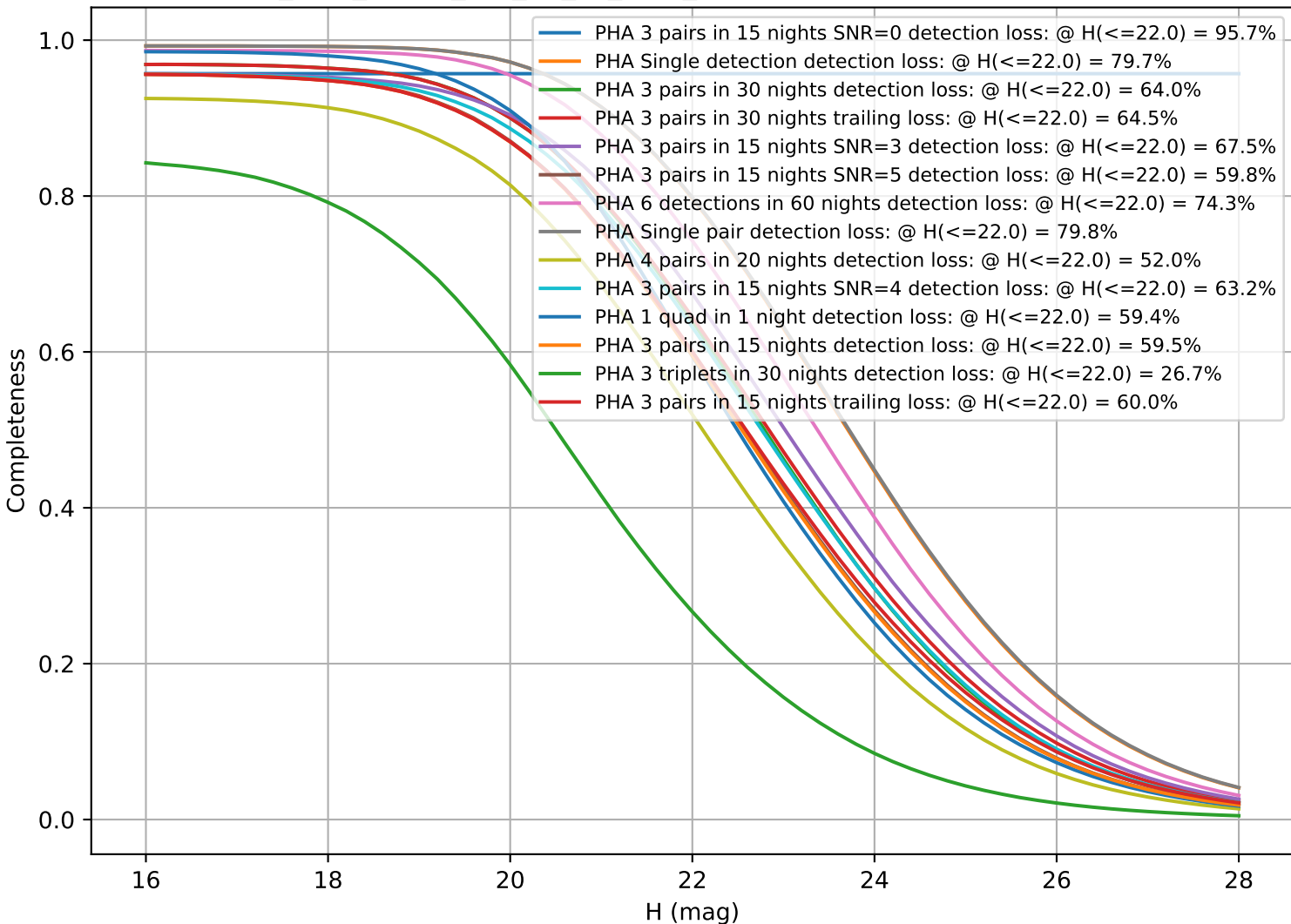
too_elab_heavy_r64_d3_gz_v3.4_10yrs: CumulativeCompleteness
