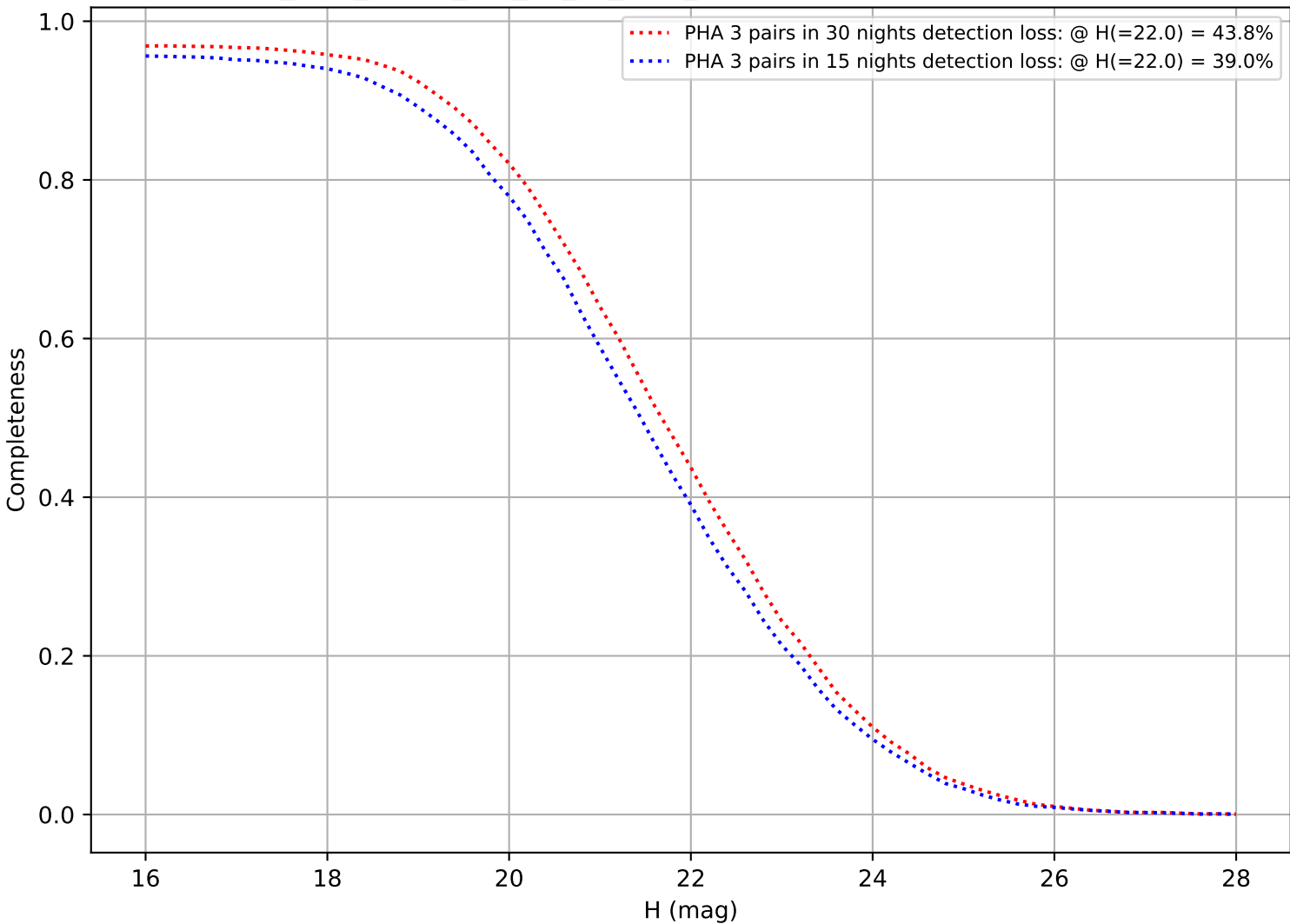
too_elab_heavy_r64_d3_gz_v3.4_10yrs: DifferentialCompleteness
