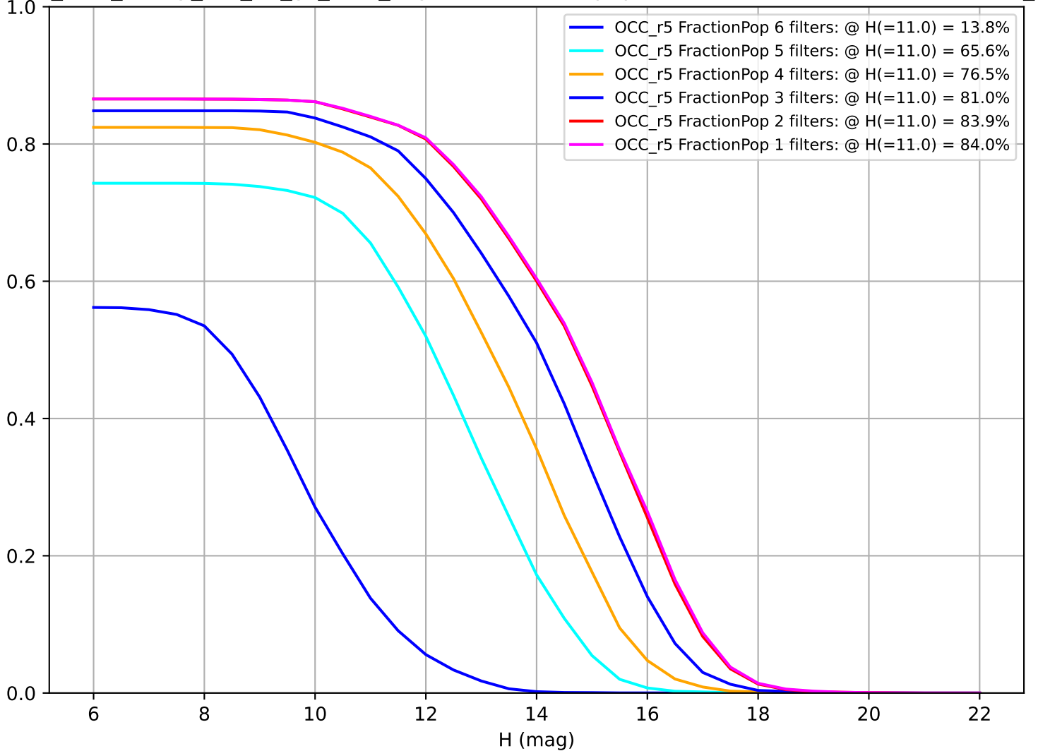
too_elab_heavy_r64_d3_gz_v3.4_10yrs: Fraction of population with colors in X filters OCC_r5
