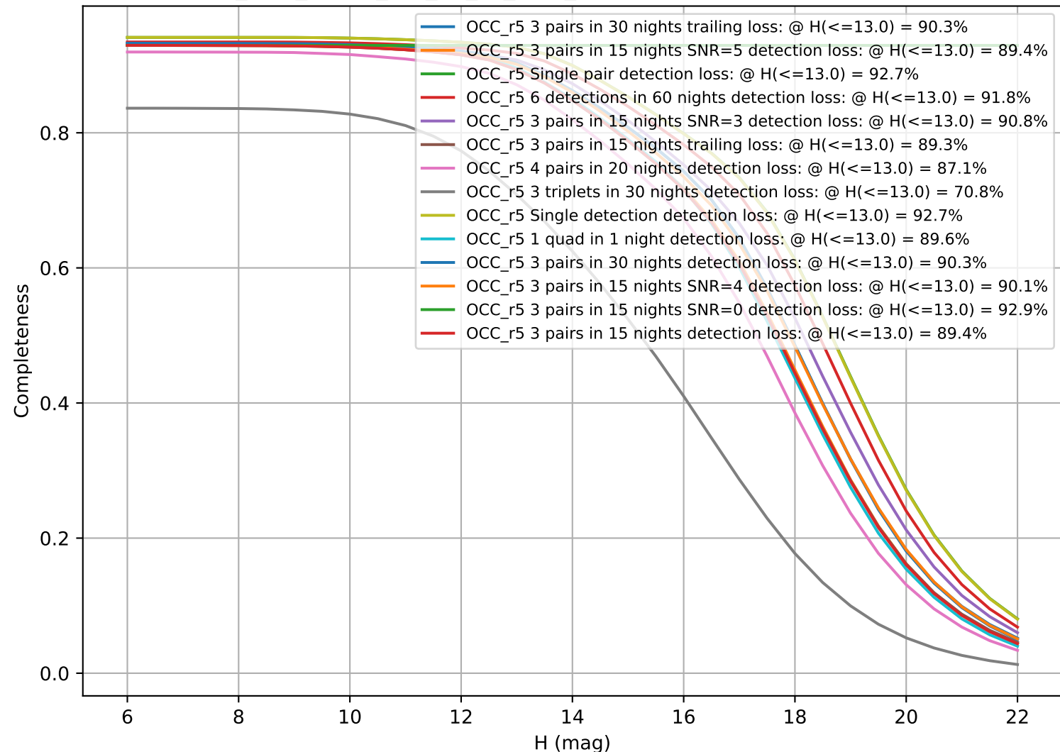
too_elab_heavy_r64_d3_gz_v3.4_10yrs: CumulativeCompleteness
