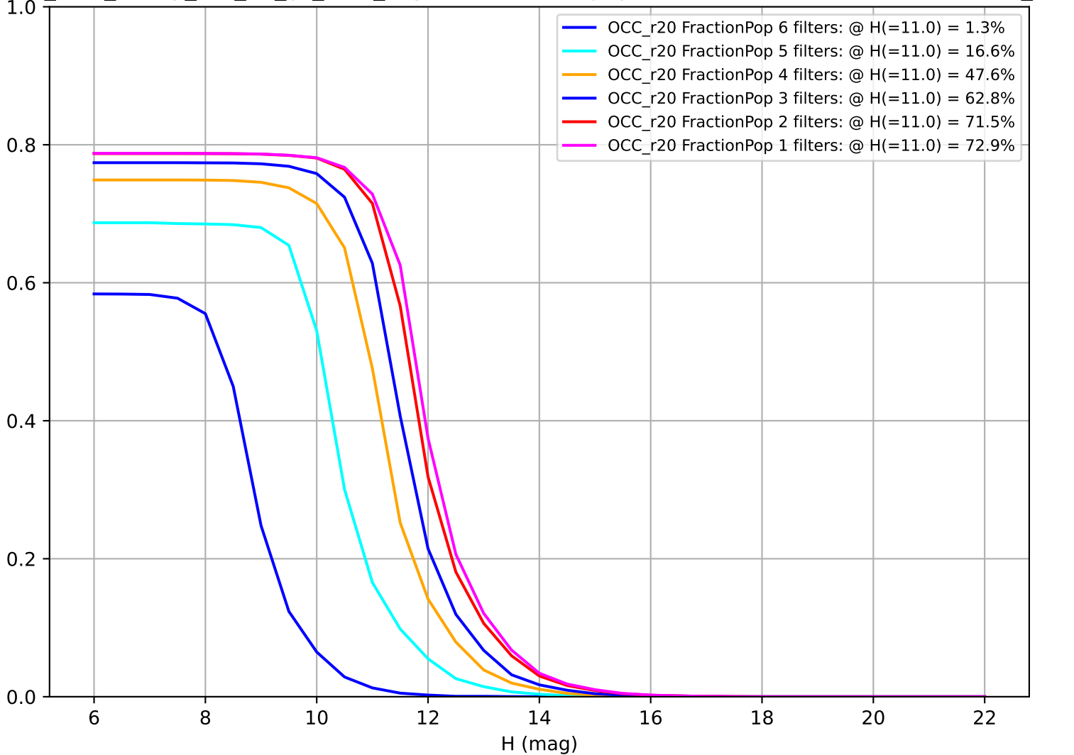
too_elab_heavy_r64_d3_gz_v3.4_10yrs: Fraction of population with colors in X filters OCC_r20
