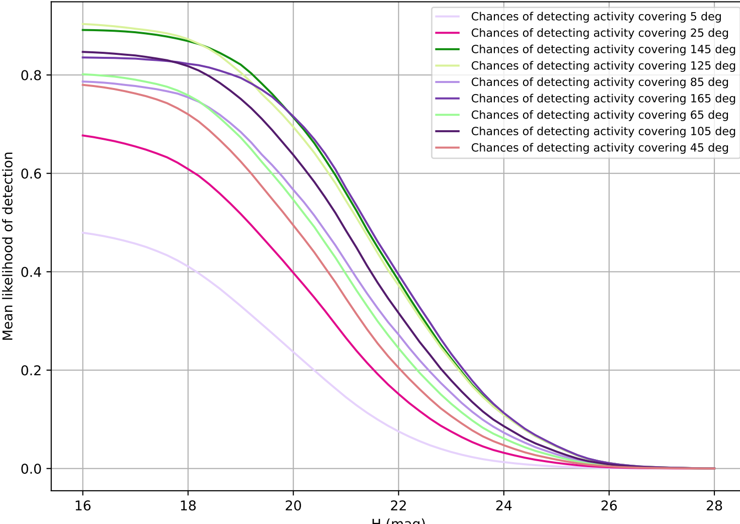
too elab heavy r64 d3 gz v3.4 10yrs NEO
