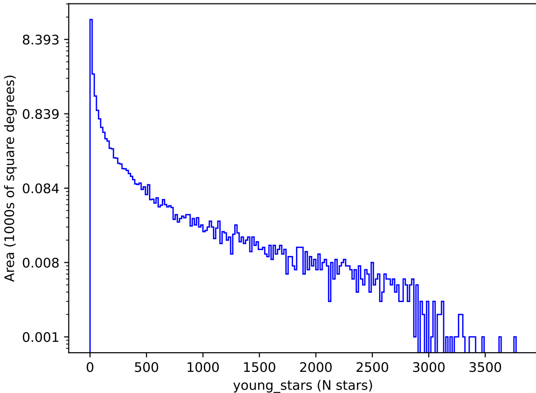
too_elab_heavy_r64_d3_gz_v3.4_10yrs : young_stars
