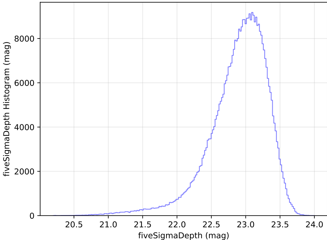
too_elab_heavy_r64_d3_gz_v3.4_10yrs z: fiveSigmaDepth Histogram
