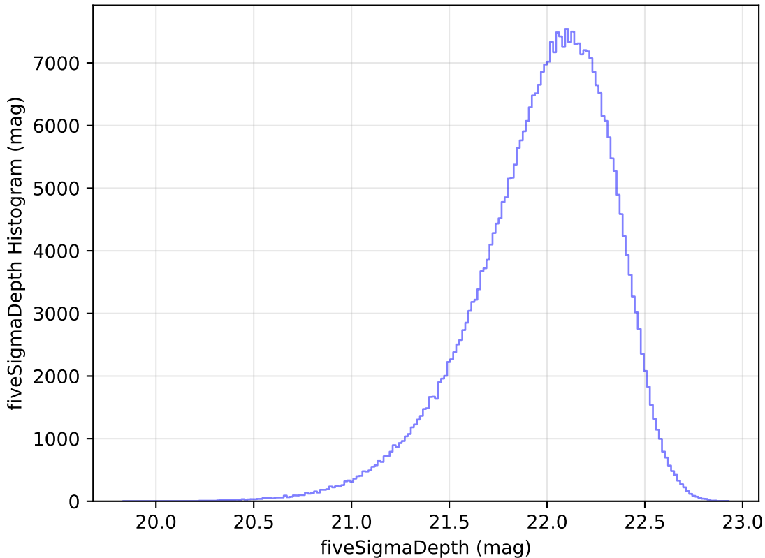
too_elab_heavy_r64_d3_gz_v3.4_10yrs y: fiveSigmaDepth Histogram
