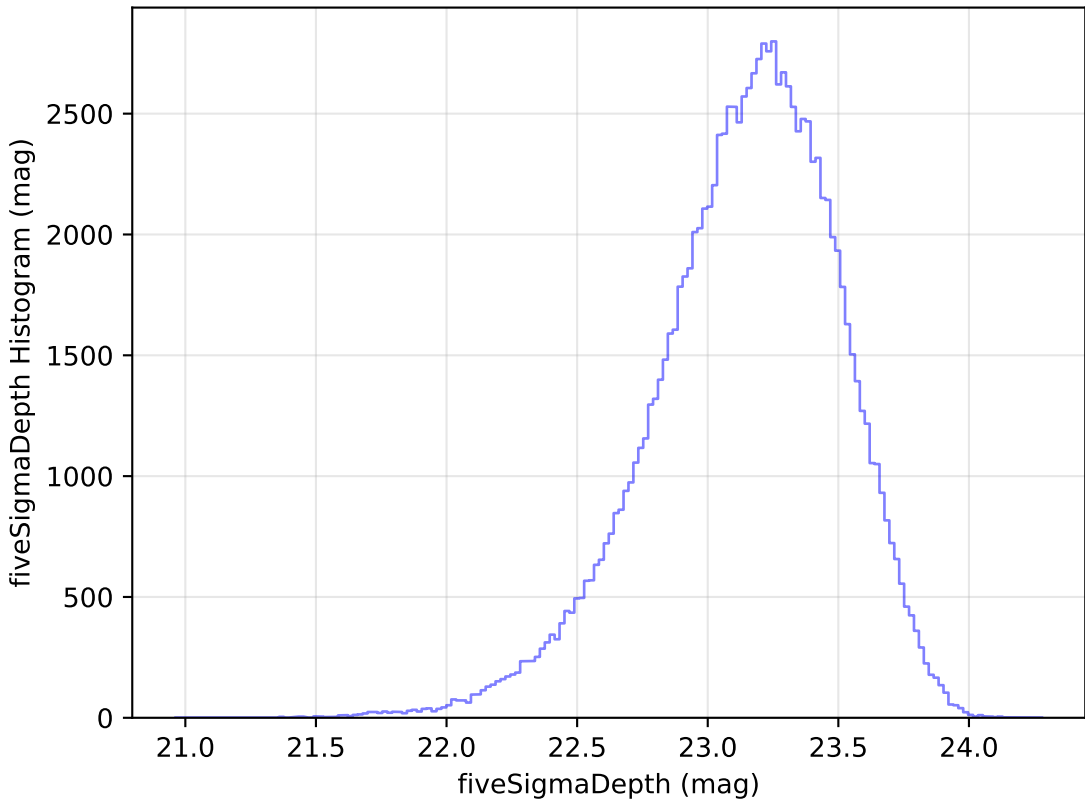
too_elab_heavy_r64_d3_gz_v3.4_10yrs u: fiveSigmaDepth Histogram
