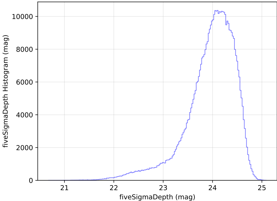
too_elab_heavy_r64_d3_gz_v3.4_10yrs r: fiveSigmaDepth Histogram
