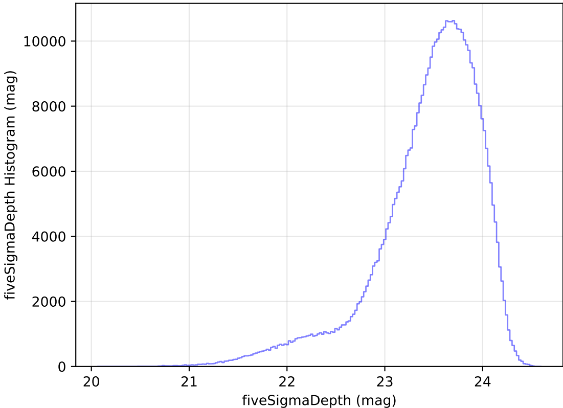
too_elab_heavy_r64_d3_gz_v3.4_10yrs i: fiveSigmaDepth Histogram
