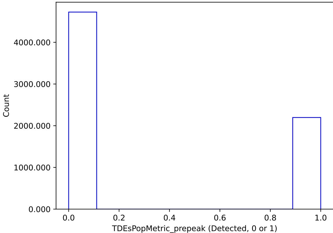
too_elab_heavy_r64_d3_gz_v3.4_10yrs : TDEsPopMetric_prepeak
