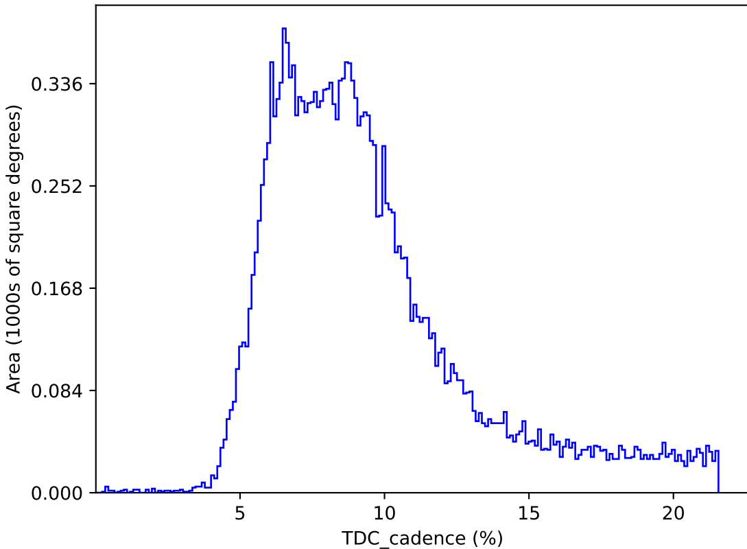
too_elab_heavy_r64_d3_gz_v3.4_10yrs : TDC_cadence
