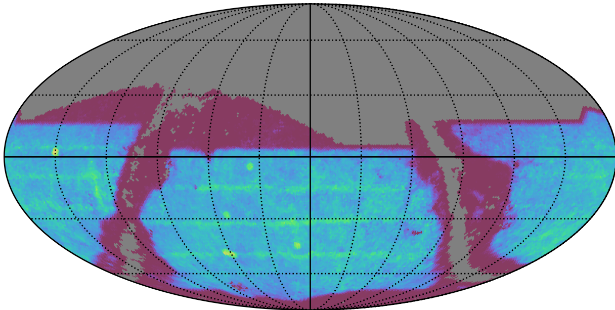
too_elab_heavy_r64_d3_gz_v3.4_10yrs : SNSLMetric
