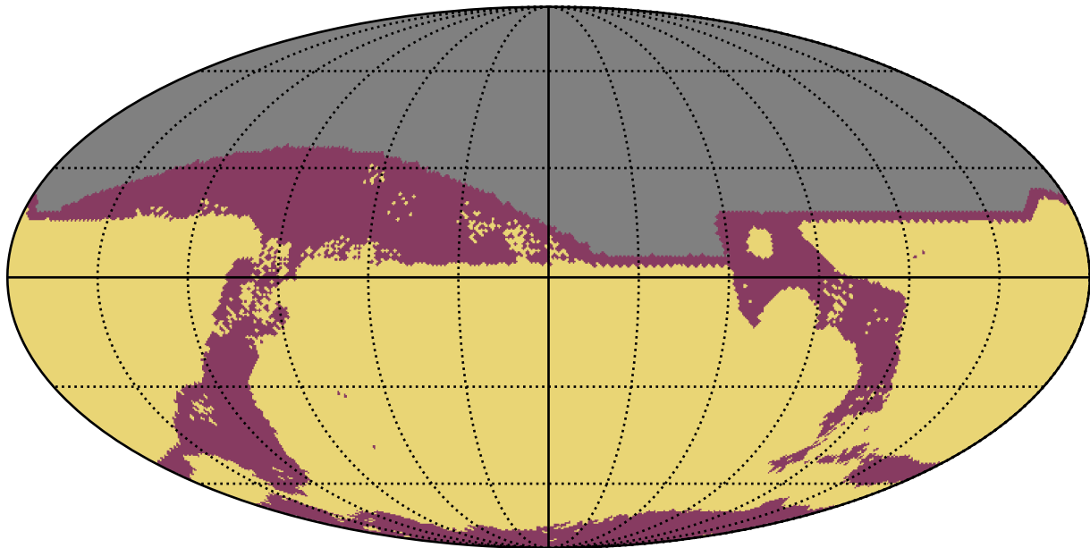
too_elab_heavy_r64_d3_gz_v3.4_10yrs : RapidRevisits
