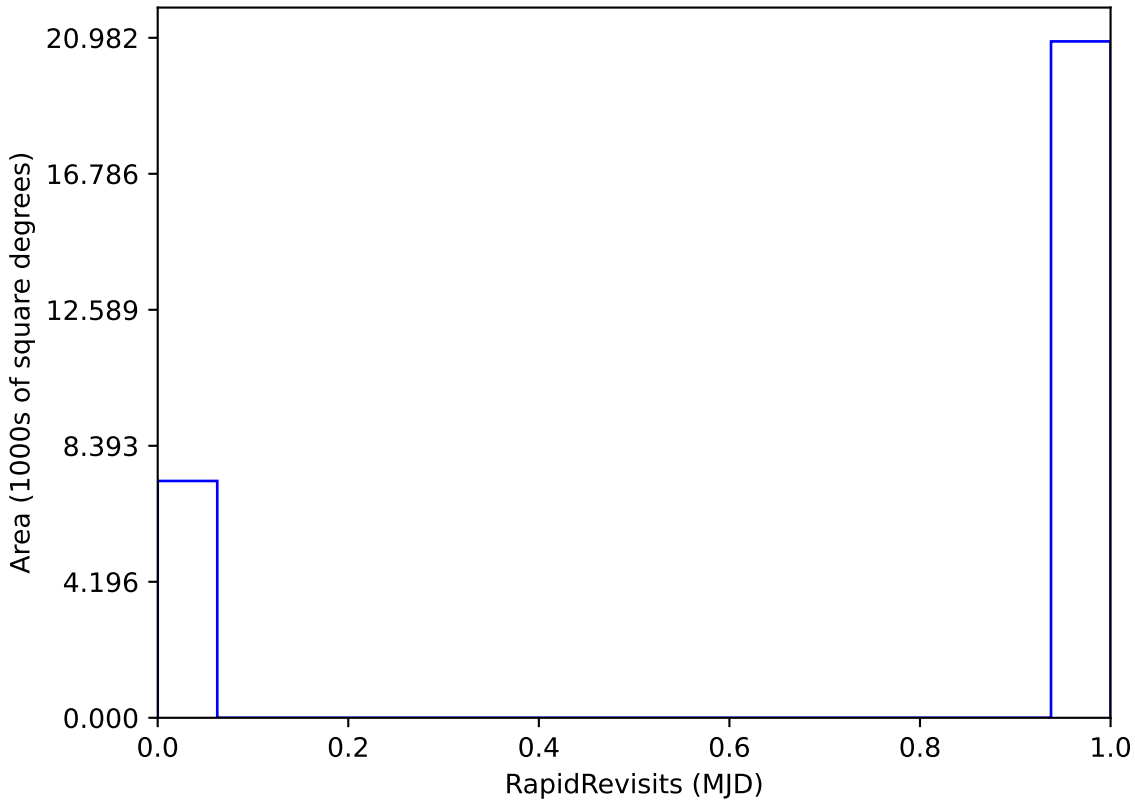
too_elab_heavy_r64_d3_gz_v3.4_10yrs : RapidRevisits
