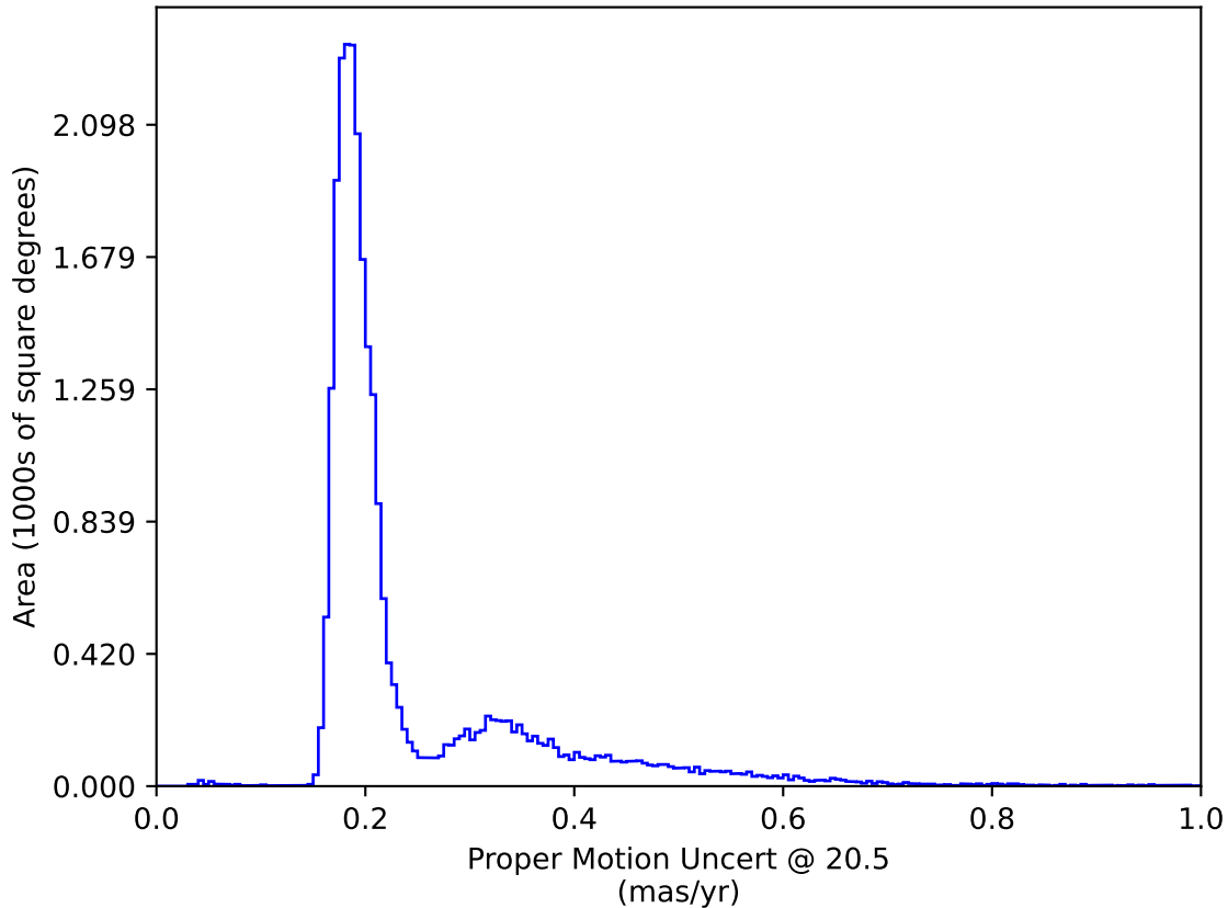
too_elab_heavy_r64_d3_gz_v3.4_10yrs : Proper Motion Uncert @ 20.5
