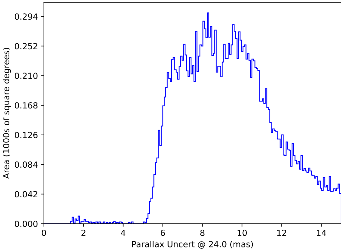
too_elab_heavy_r64_d3_gz_v3.4_10yrs : Parallax Uncert @ 24.0
