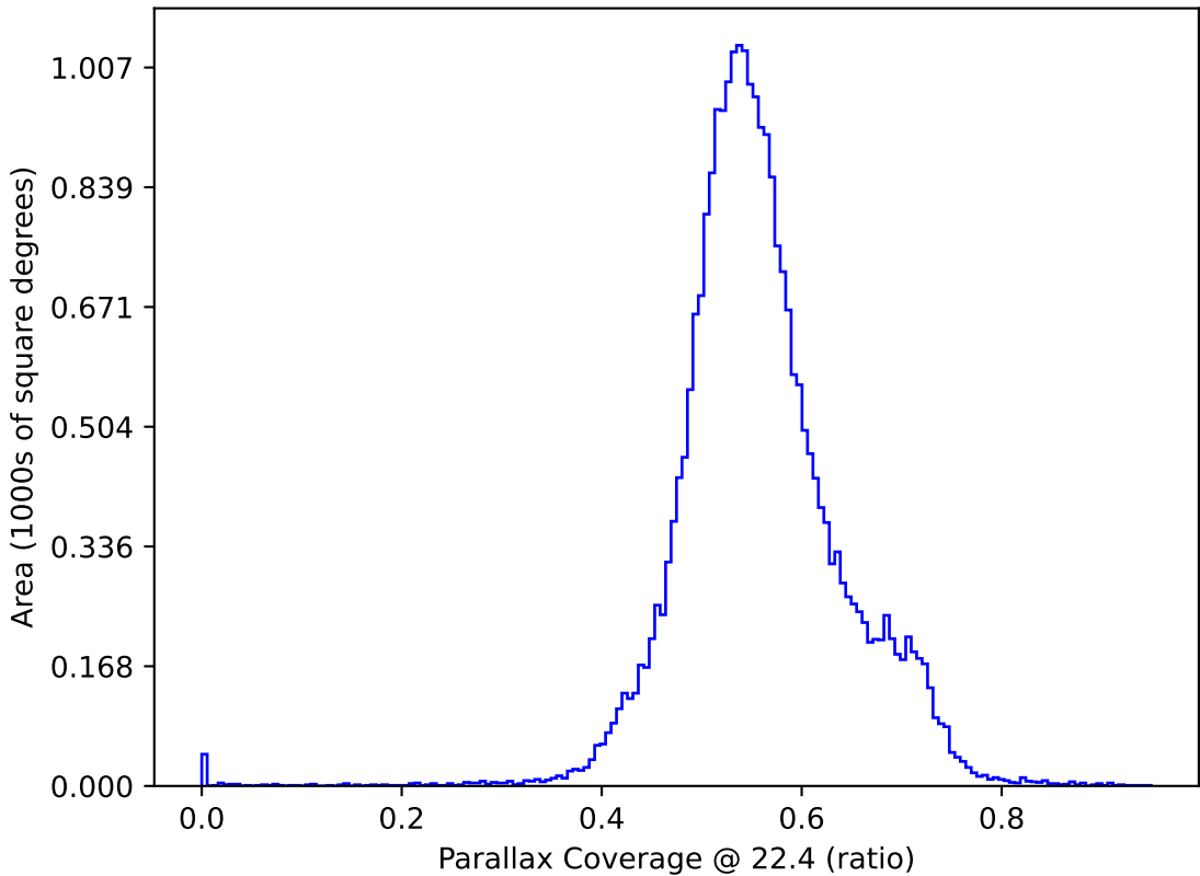
too_elab_heavy_r64_d3_gz_v3.4_10yrs : Parallax Coverage @ 22.4
