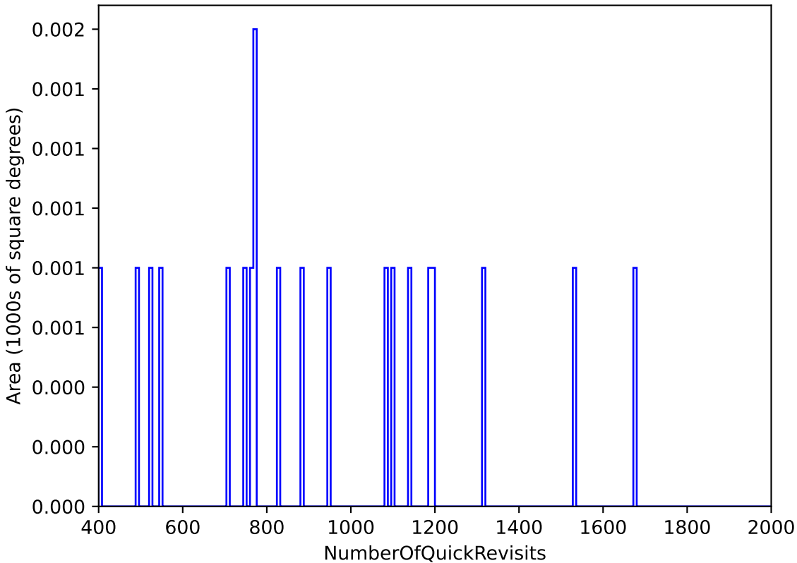
too_elab_heavy_r64_d3_gz_v3.4_10yrs : NumberOfQuickRevisits
