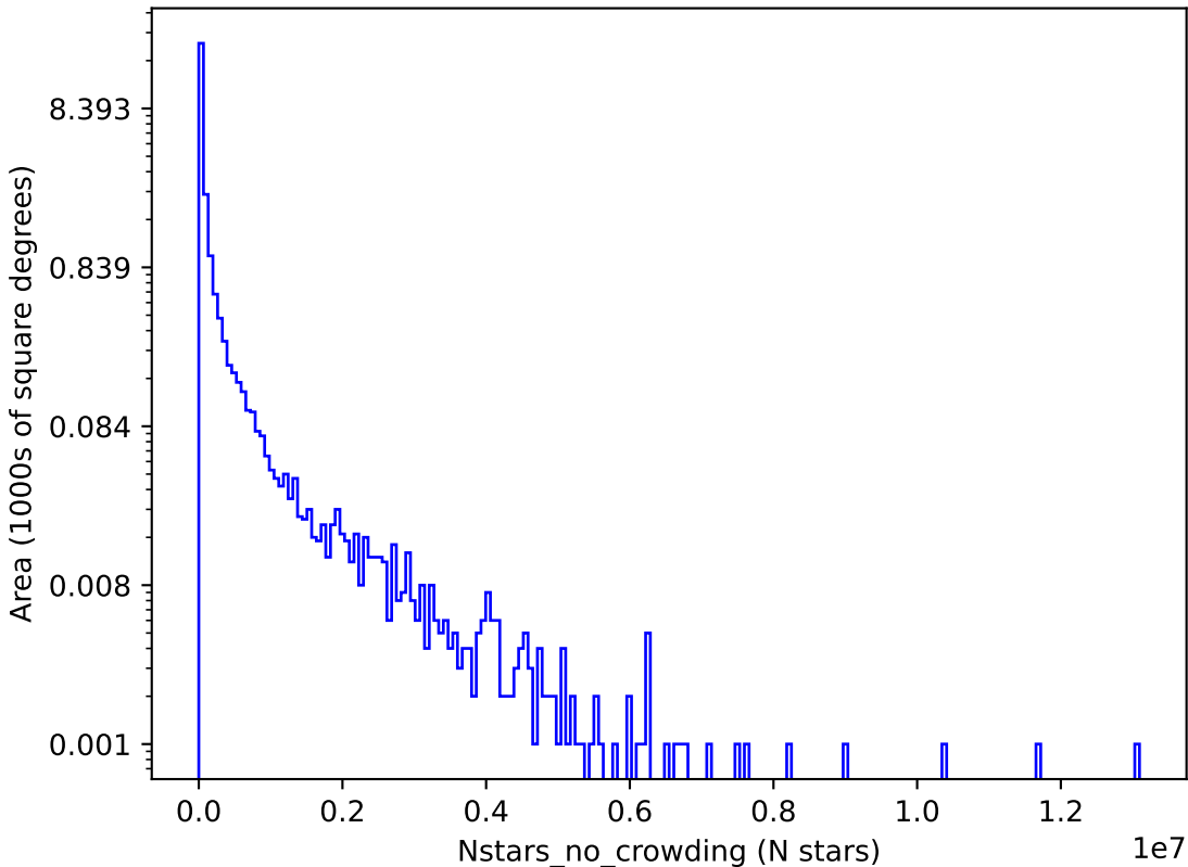
too_elab_heavy_r64_d3_gz_v3.4_10yrs g: Nstars_no_crowding
